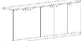
5Shutter- Back Credenza Low Height 2100 X 400 X 625 - UM-OBSEL13 2100 X 400 X 750 - UM-OBSEL14 2100 X 400 X 900 - UM-OBSEL15 2400 X 400 X 625 - UM-OBSEL16 2400 X 400 X 750 - UM-OBSEL17 2400 X 400 X 900 - UM-OBSEL18
