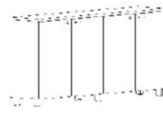
4Shutter- Back Credenza Low Height 1800 X 400 X 625 - UM-OBSFL07 1800 X 400 X 750 - UM-OBSFL08 1800 X 400 X 900 - UM-OBSFL09 2000 X 400 X 625 - UM-OBSFL10 2000 X 400 X 750 - UM-OBSFL11 2000 X 400 X 900 - UM-OBSFL12 1800 X 400 X 1200 - UM-OBSFL23 2000 X 400 X 1200 - UM-OBSFL24
