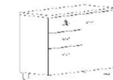
File Drawer Pedestal Unit 900 X 400 X 625 - UM-OSCFH01 900 X 400 X 750 - UM-OSCFH02 1050 X 400 X 625 - UM-OSCFH03 1050 X 400 X 750 - UM-OSCFH04 900 X 450 X 625 - UM-OSCFH05 900 X 450 X 750 - UM-OSCFH06 1050 X 450 X 625 - UM-OSCFH07 1050 X 450 X 750 - UM-OSCFH08
